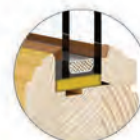
Retro profile with Retro glazing beads available
